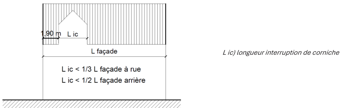
Figure 6 : Interruption de corniche
